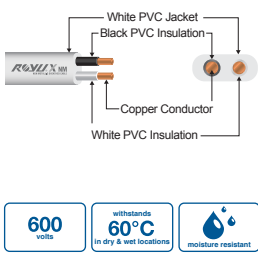
ROYUX NM Non Metallic Sheathed Cable
